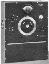
FIGURE 1. Above the frequency-control dial of the wave analyzer is the voltmeter shown in FIGURE 2. At the left is the meter multiplier
